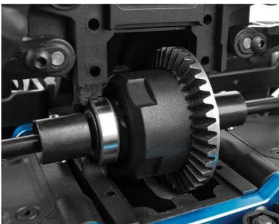
Oil-filled front, center, and rear differentials with sintered powdered metal ring and pinion gears.
