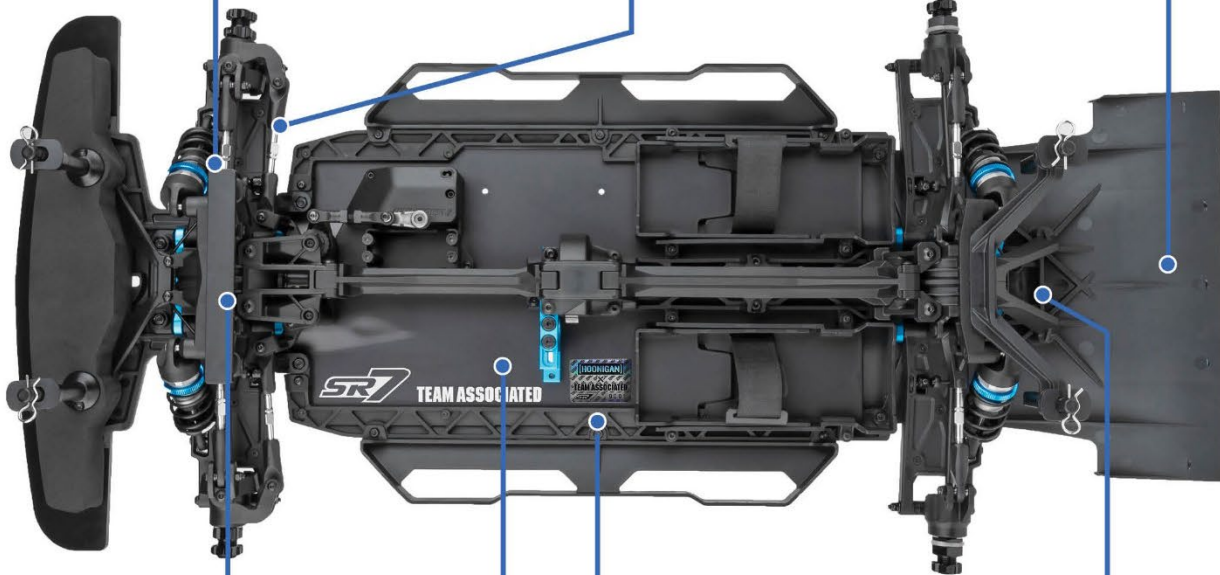
Oil-filled front, center, and rear differentials with sintered powdered metal ring and pinion gears.
