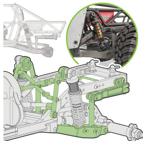
GKS trailing arms in green
