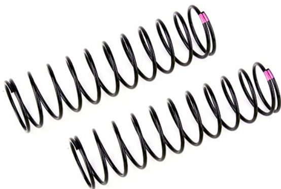
(Pictured: #81233 Rear Springs V2, pink, 3.7 lb/in, L86, 12.00T, 1.6D.)
