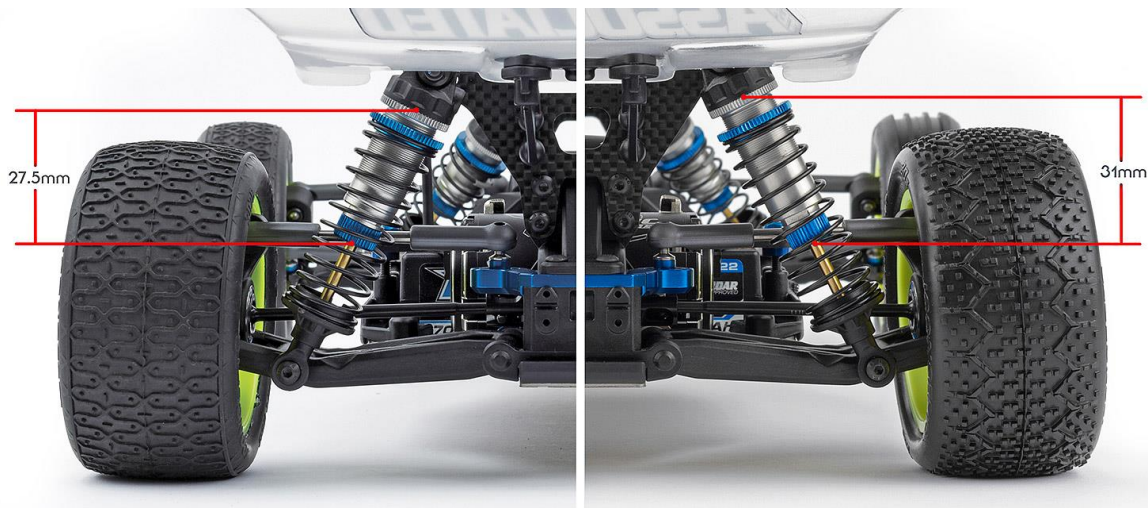
For comparison: Left: standard #91665 shock tower. Right: optional #91666 shock tower.
