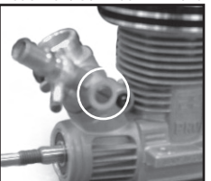
Adjust so the screw is even with the carb body
