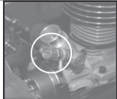
High Speed Mixture: 3 turns out Clockwise = Leaner Counterclockwise = Richer
