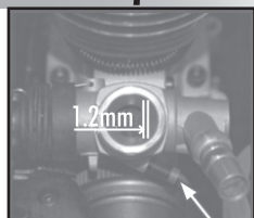
Idle Speed: .050" (1.2mm) Adjust Idle Screw until .7mm is obtained.
