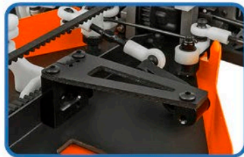
Floating servo mount
