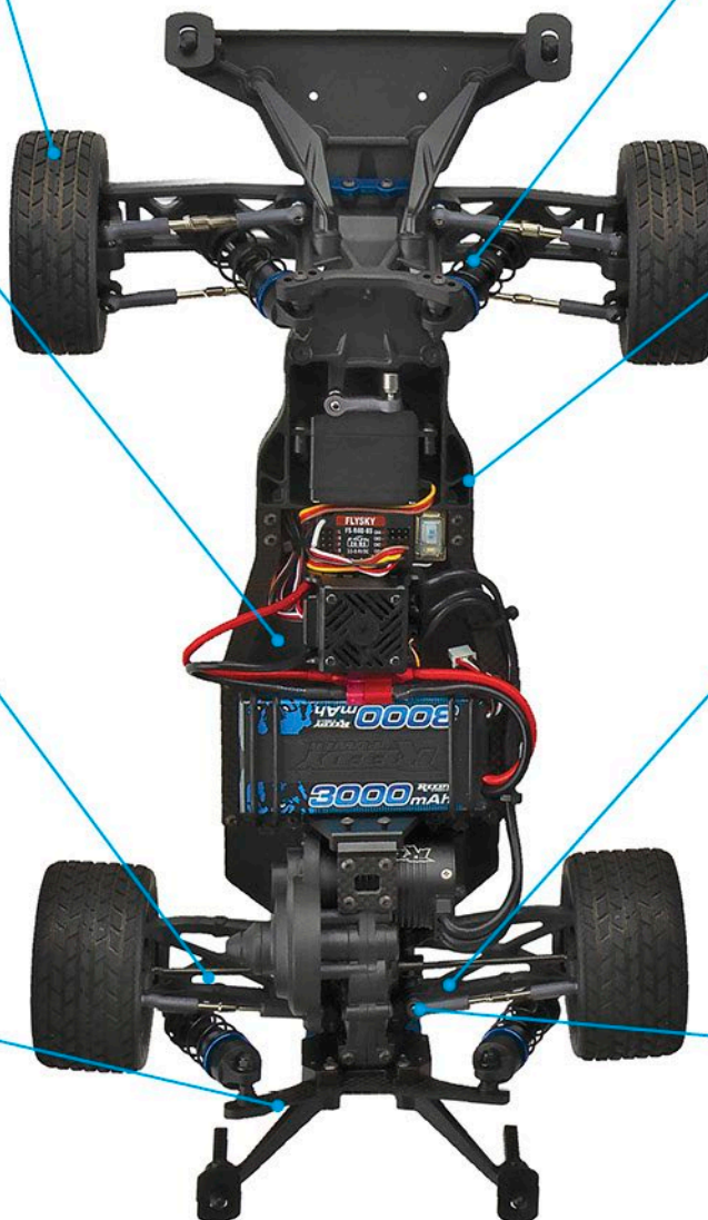
Adjustable suspension geometry with aluminum 12mm coil-over shock absorbers
