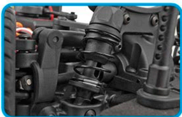
Coil-over shock absorbers
