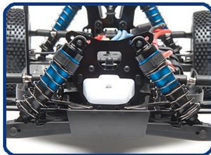
RC8.2 racing suspension geometry
