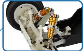
Top loading, gold anodized racing shocks.
