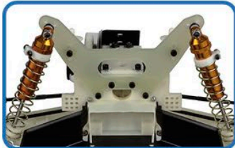
Long travel, fiberglass rear shock tower. 1-piece rugged nylon bulkhead.
