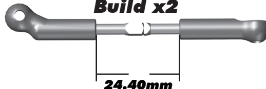
Steering Build x2
