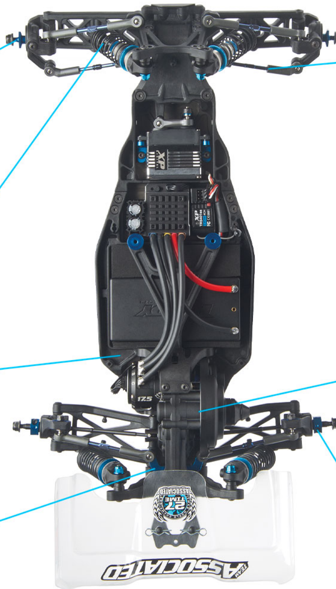
Lightweight, hard-anodized aluminum chassis with centralized mass, mid-motor
