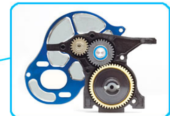
3-gear transmission with lightweight V2 aluminum top shaft included
