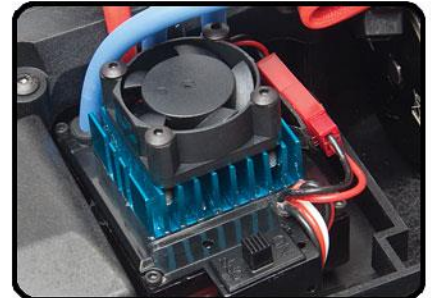
XP water-resistant ESC with high-current T-plug connector
