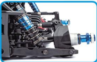
Four oil-filled shocks designed for smooth and consistent operation
