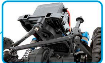
Chassis Mounted Steering (CMS) servo
