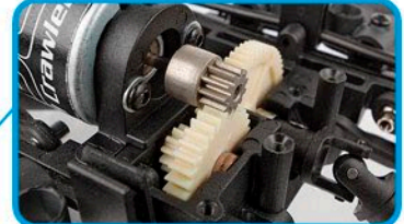
13.98:1 ratio 3-gear transmission with integrated motor mount
