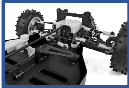
Floating Servo Mount
