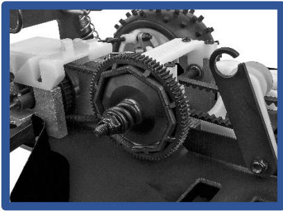
Slipper Clutch
